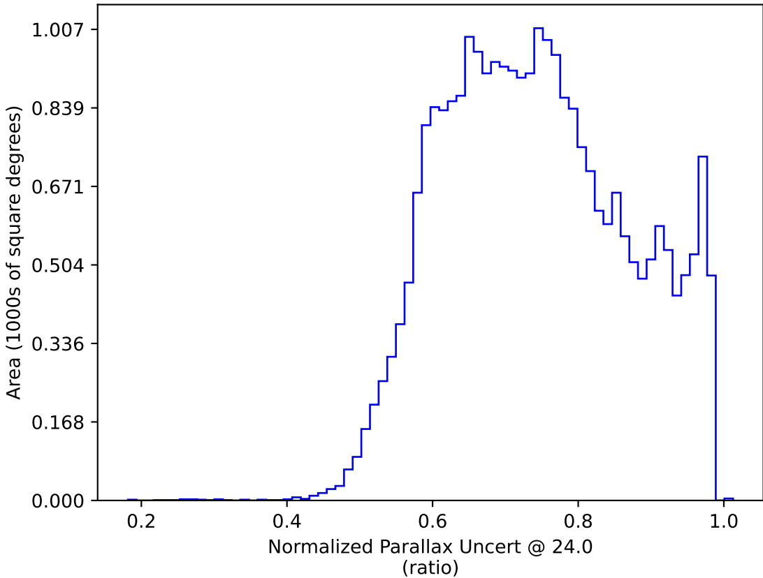
noroll_mjdp120_v3.4_10yrs : Normalized Parallax Uncert @ 24.0
