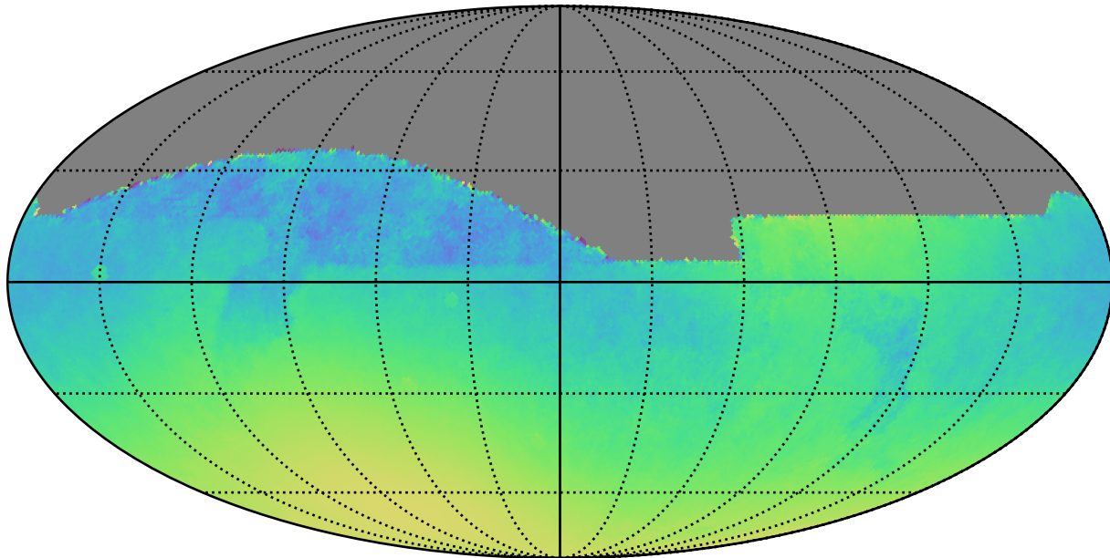
noroll_mjdp120_v3.4_10yrs : Normalized Parallax Uncert @ 22.4
