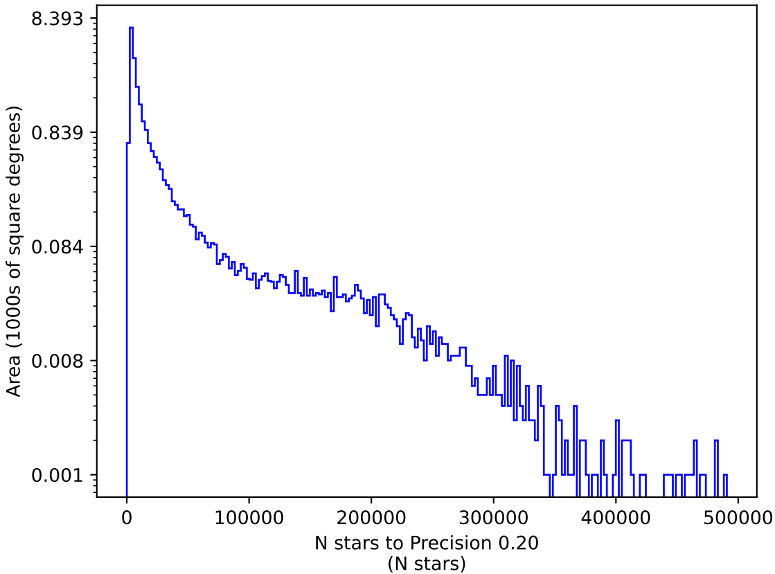
noroll_mjdp120_v3.4_10yrs u: N stars to Precision 0.20
