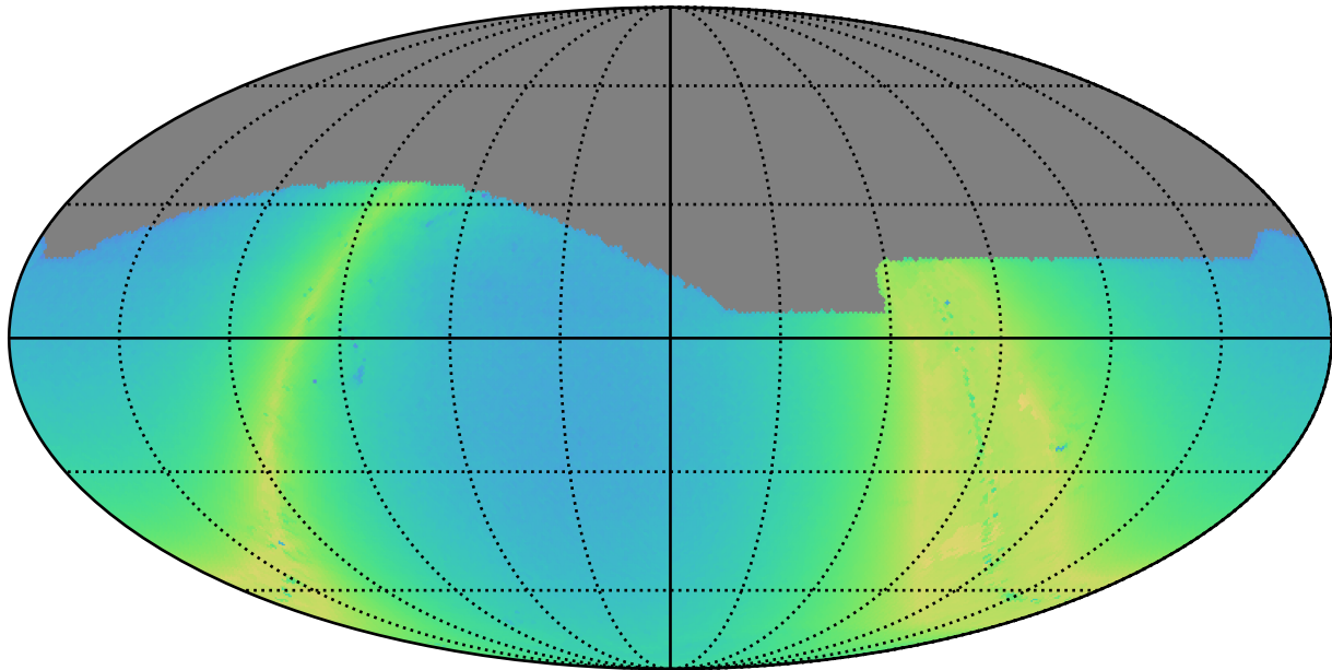
noroll_mjdp120_v3.4_10yrs i: N stars to Precision 0.20
