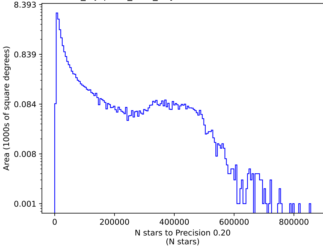
noroll_mjdp120_v3.4_10yrs i: N stars to Precision 0.20
