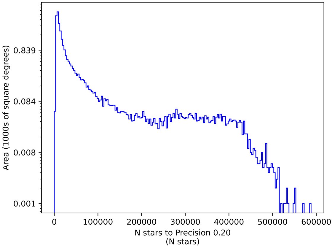
noroll_mjdp120_v3.4_10yrs g: N stars to Precision 0.20
