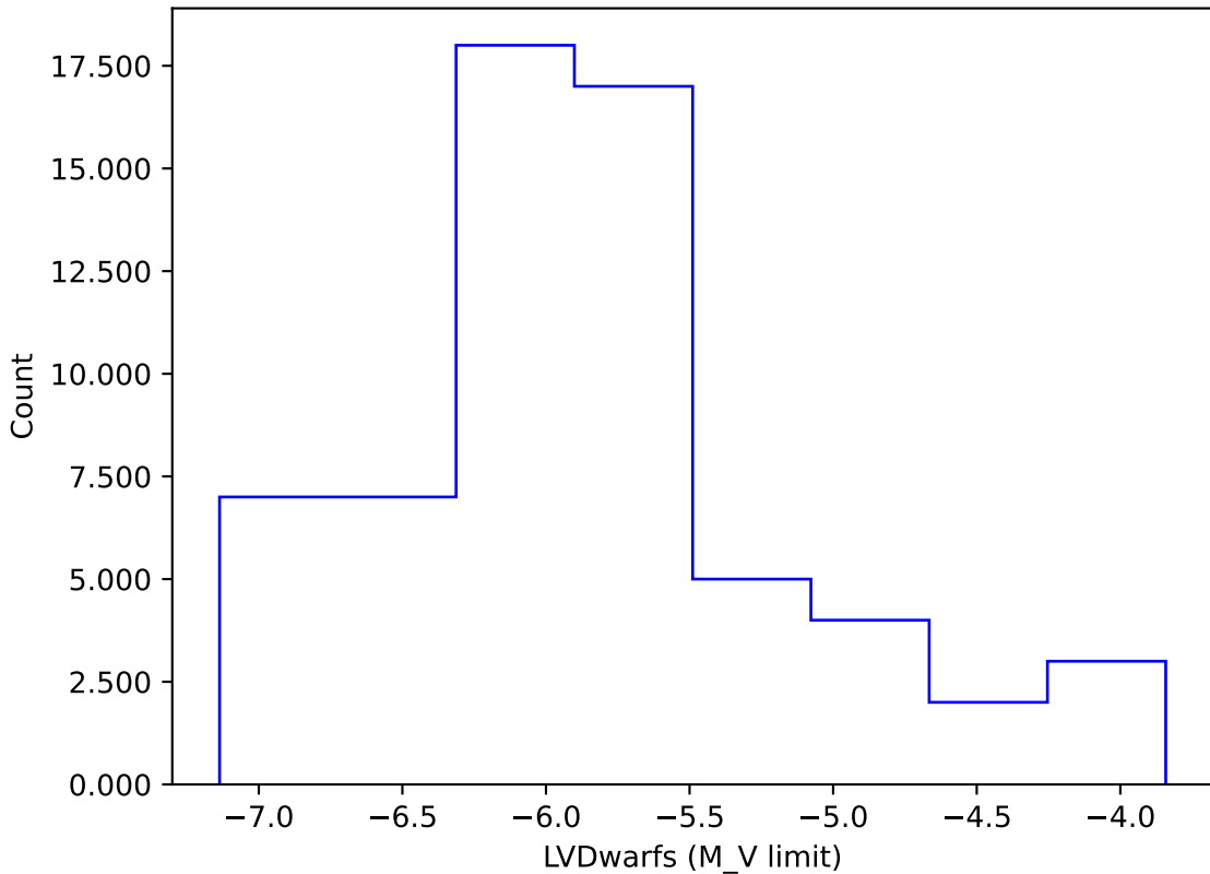
noroll_mjdp120_v3.4_10yrs gi: LVDwarfs
