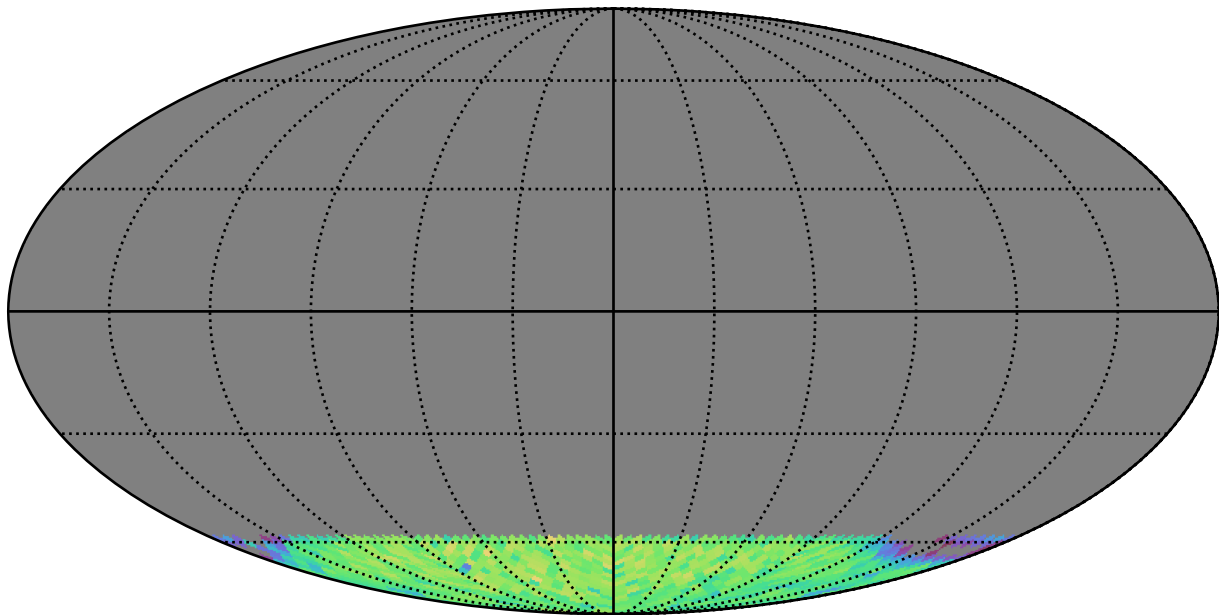
noroll_mjdp120_v3.4_10yrs gi SCP: LVDwarfs
