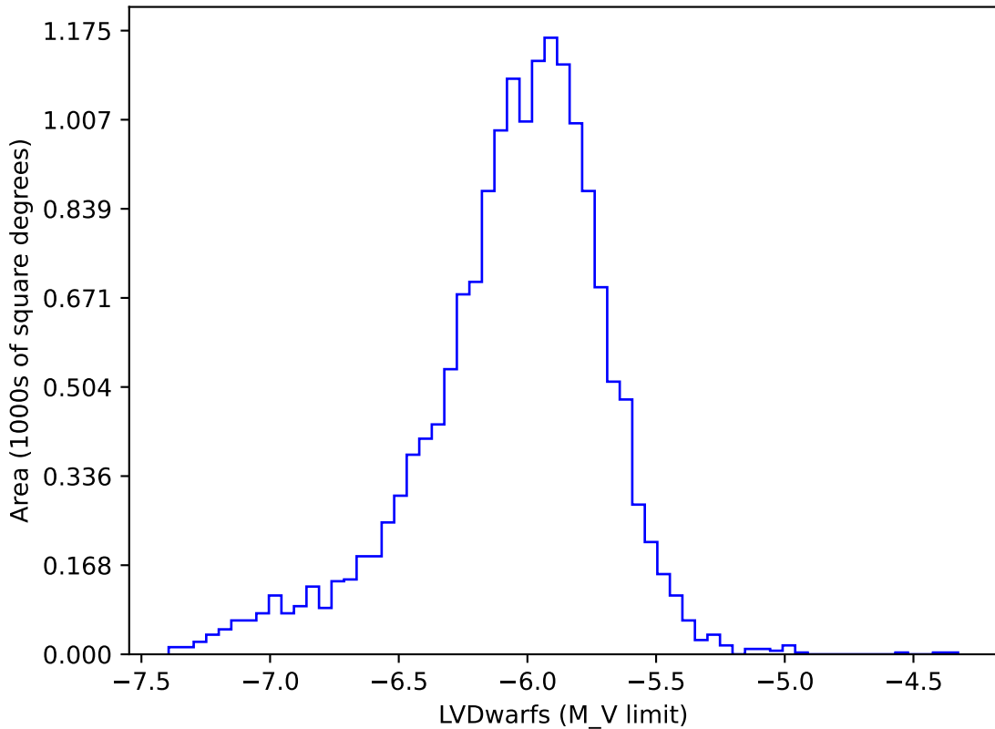
noroll_mjdp120_v3.4_10yrs gi: LVDwarfs
