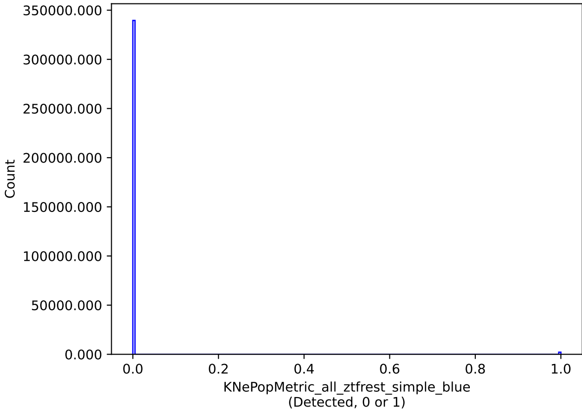
noroll_mjdp120_v3.4_10yrs all models: KNePopMetric_all_ztfrest_simple_blue
