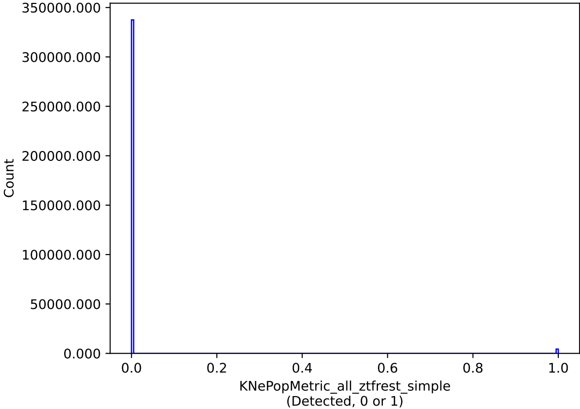
noroll_mjdp120_v3.4_10yrs all models: KNePopMetric_all_ztfrest_simple
