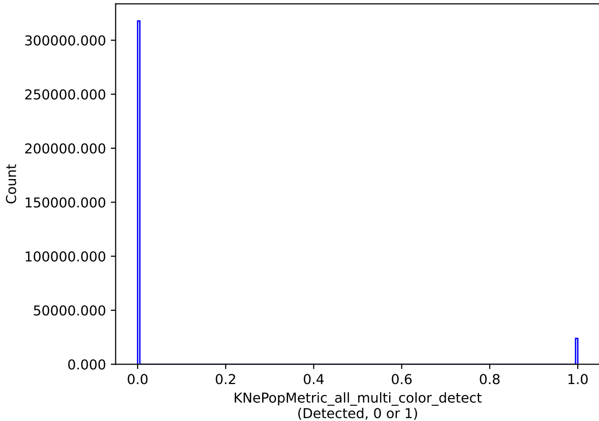
noroll_mjdp120_v3.4_10yrs all models: KNePopMetric_all_multi_color_detect
