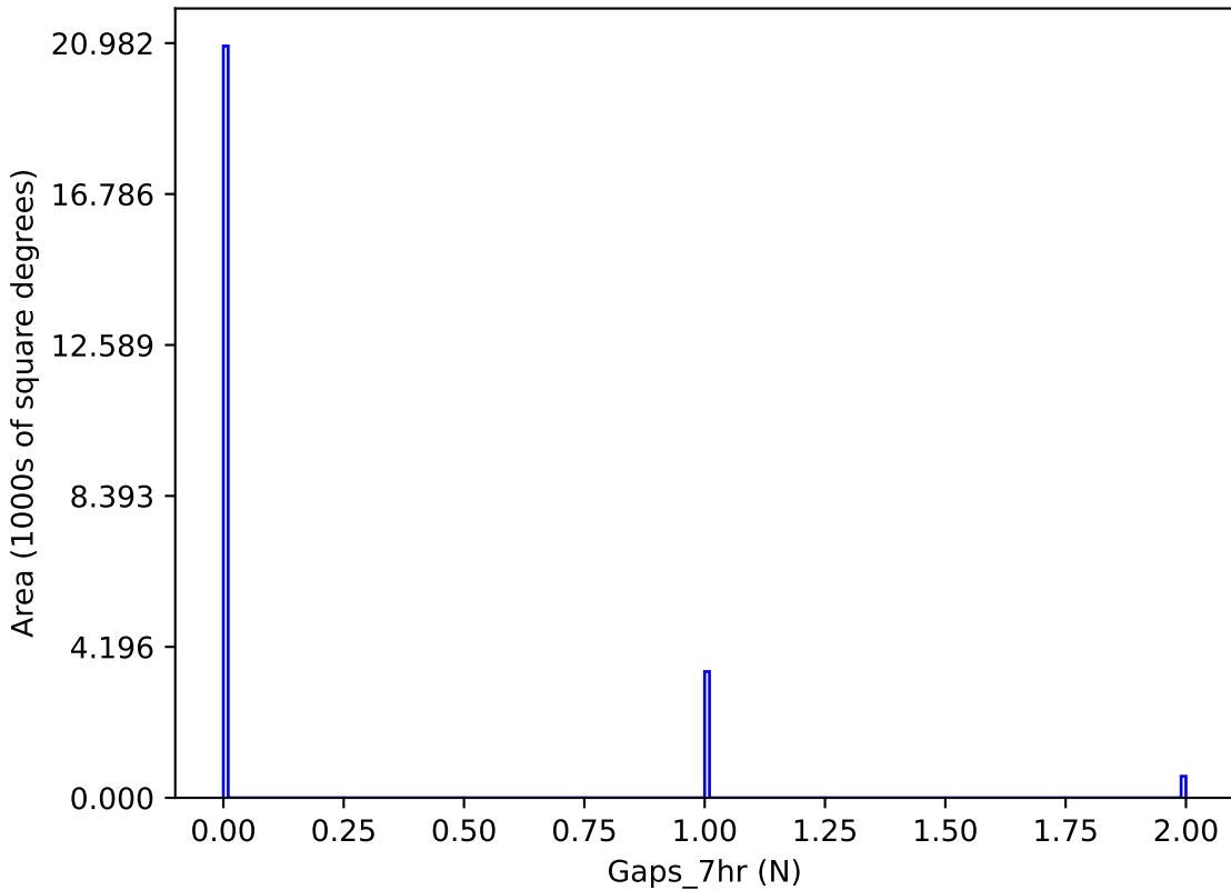
noroll_mjdp120_v3.4_10yrs y band: Gaps_7hr
