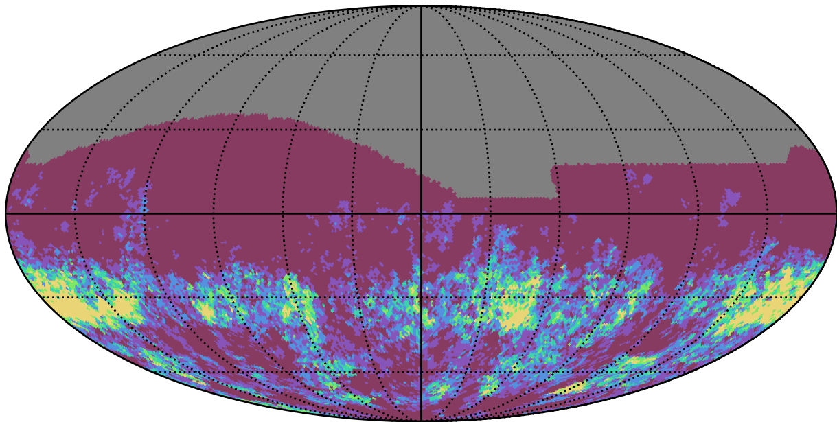
noroll_mjdp120_v3.4_10yrs r band: Gaps_7hr
