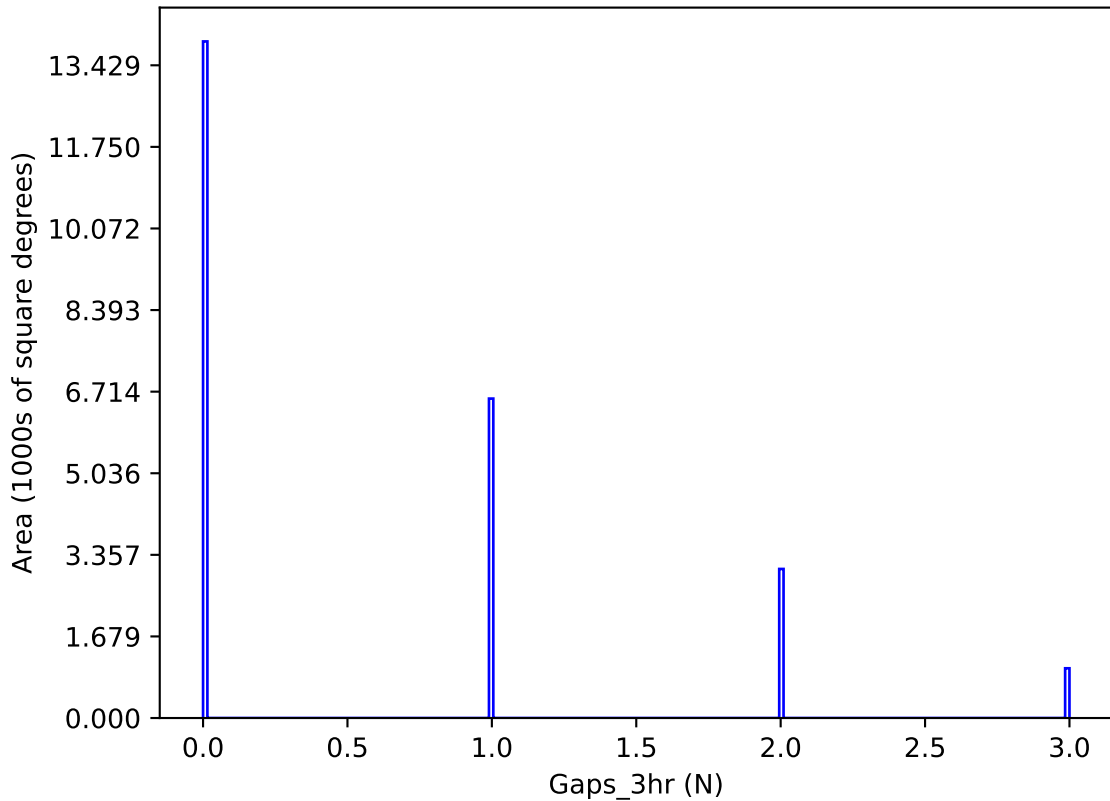
noroll_mjdp120_v3.4_10yrs y band: Gaps_3hr
