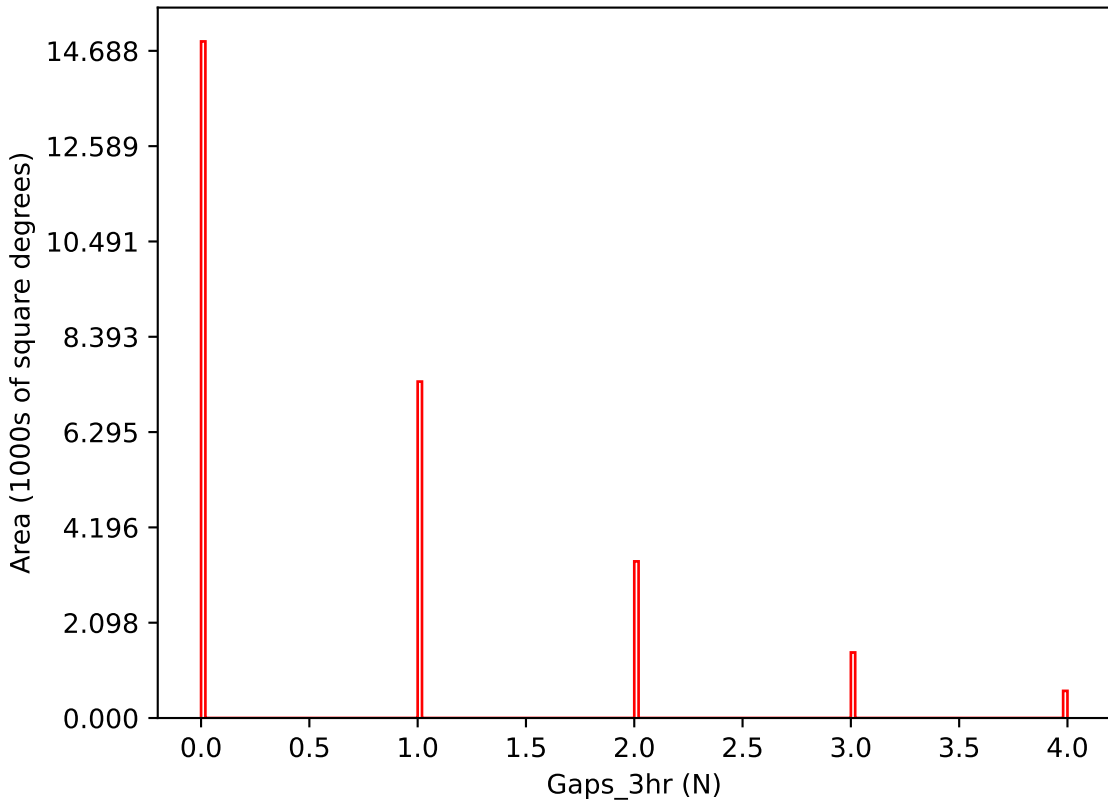
noroll_mjdp120_v3.4_10yrs i band: Gaps_3hr
