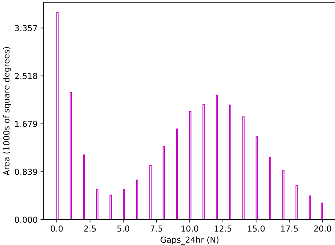
noroll_mjdp120_v3.4_10yrs z band: Gaps_24hr
