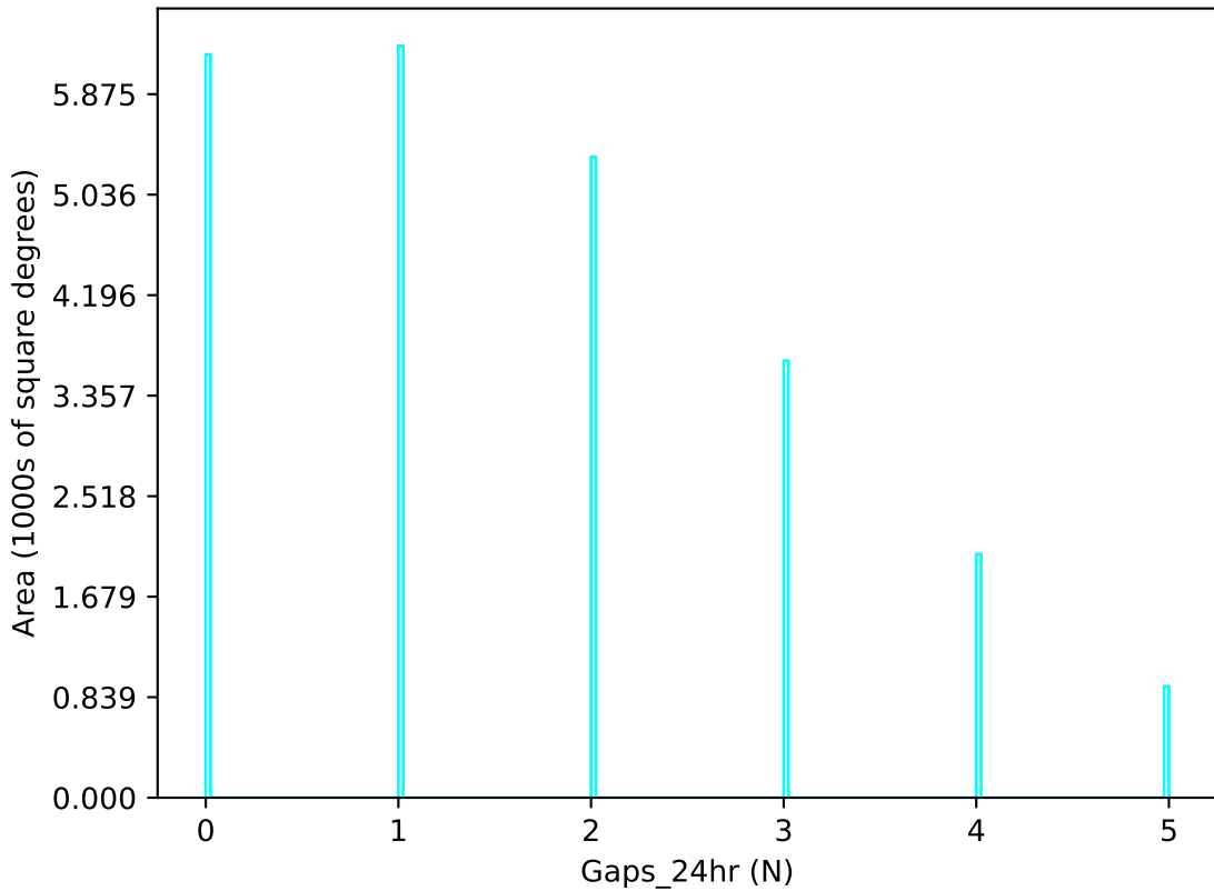
noroll_mjdp120_v3.4_10yrs u band: Gaps_24hr
