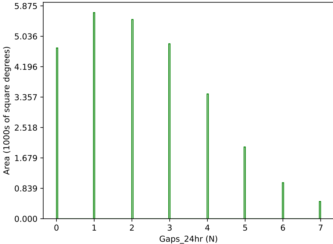
noroll_mjdp120_v3.4_10yrs g band: Gaps_24hr
