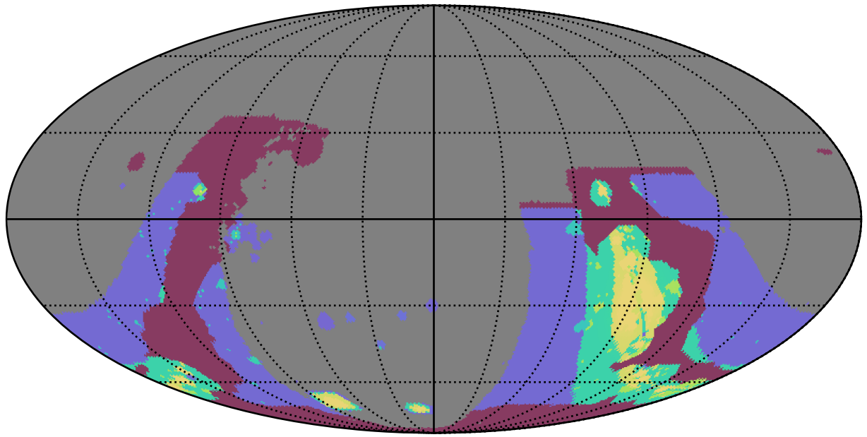
noroll_mjdp120_v3.4_10yrs : GalplaneFootprintMetric_combined_map_Tau_11_0
