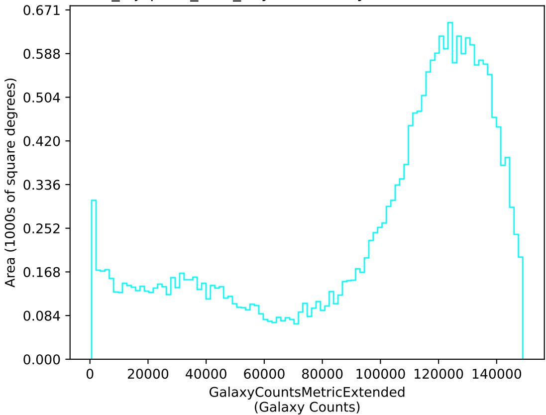
noroll_mjdp120_v3.4_10yrs u: GalaxyCountsMetricExtended
