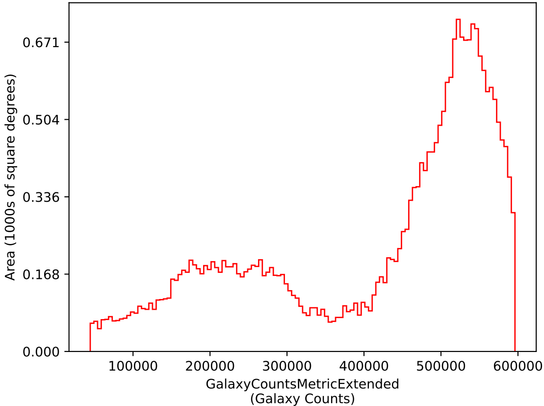
noroll_mjdp120_v3.4_10yrs i: GalaxyCountsMetricExtended
