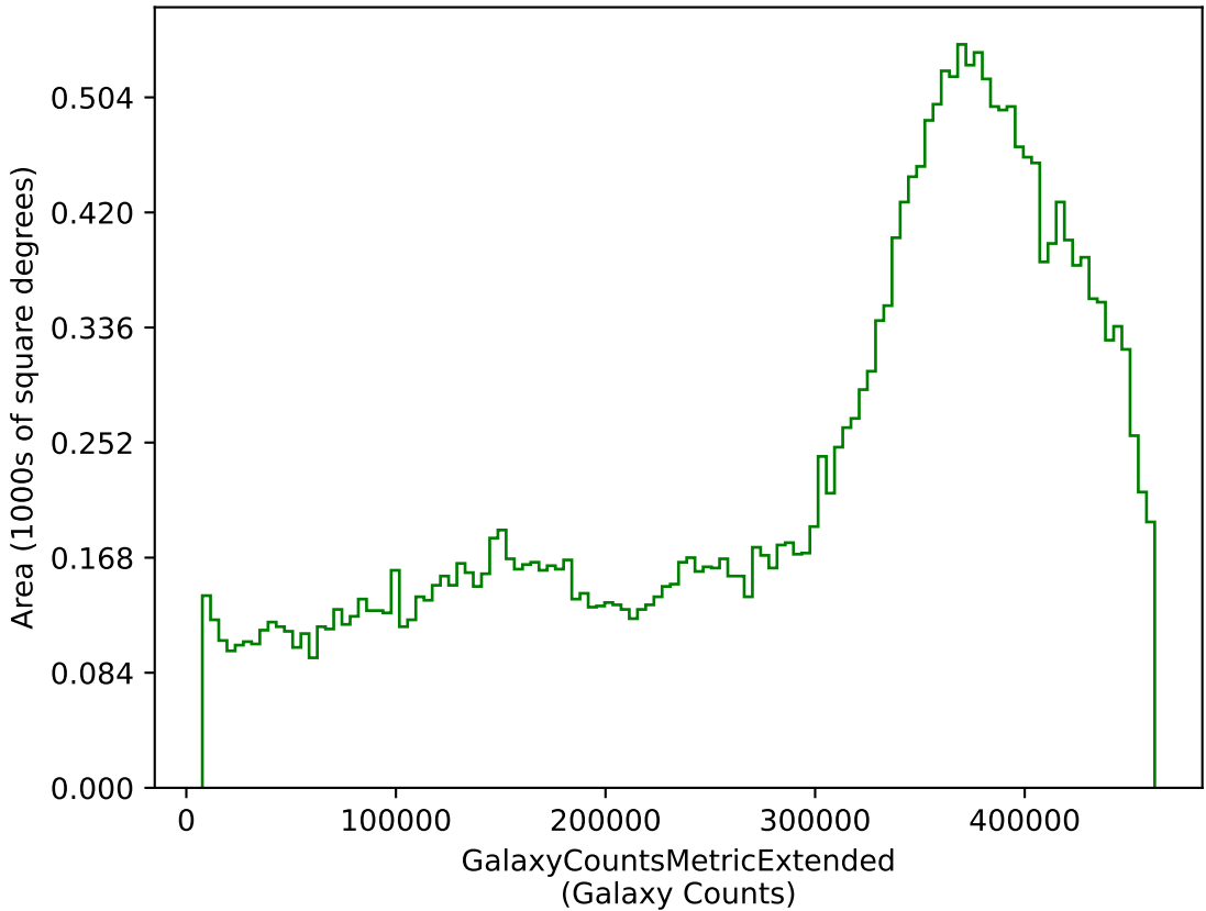
noroll_mjdp120_v3.4_10yrs g: GalaxyCountsMetricExtended
