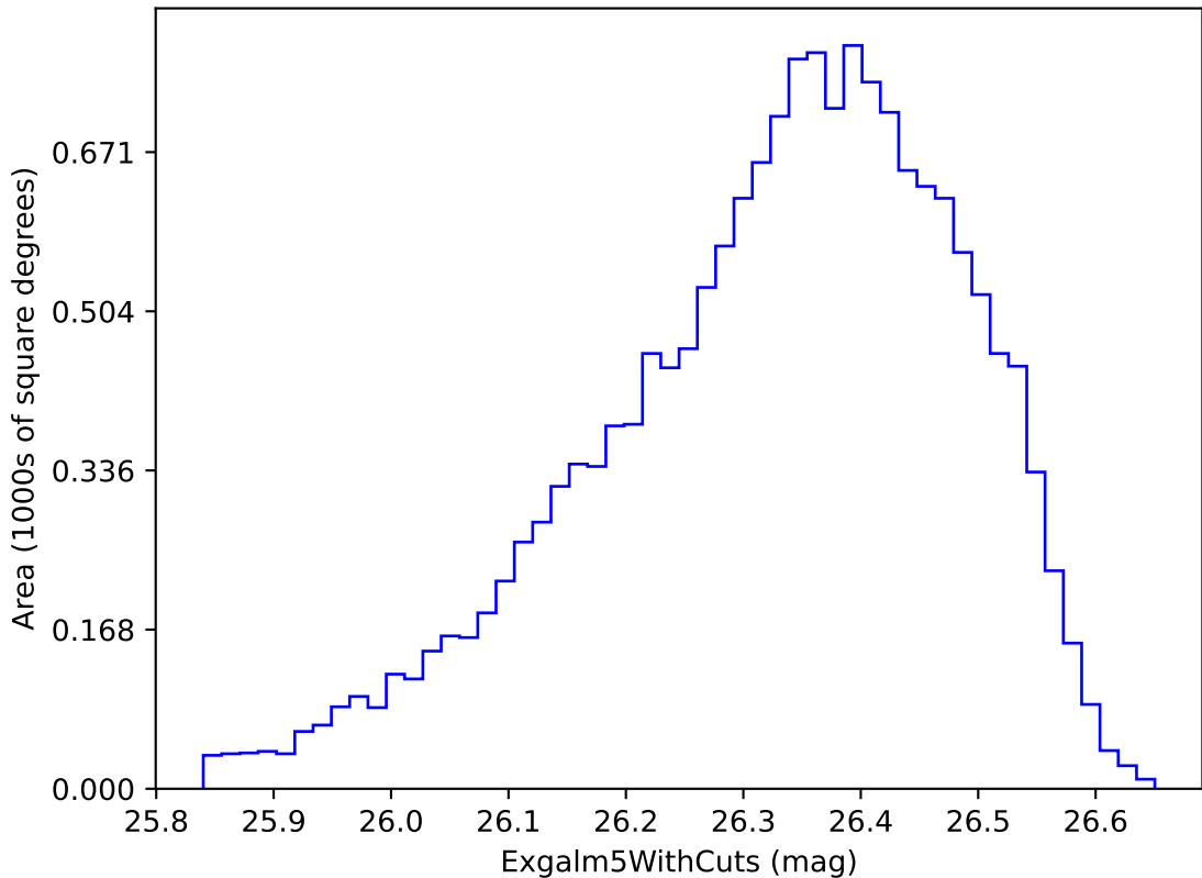
noroll_mjdp120_v3.4_10yrs i band non-DD year 9: ExgalM5WithCuts
