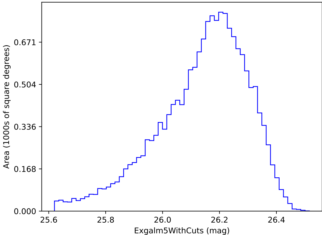
noroll_mjdp120_v3.4_10yrs i band non-DD year 6: ExgalM5WithCuts
