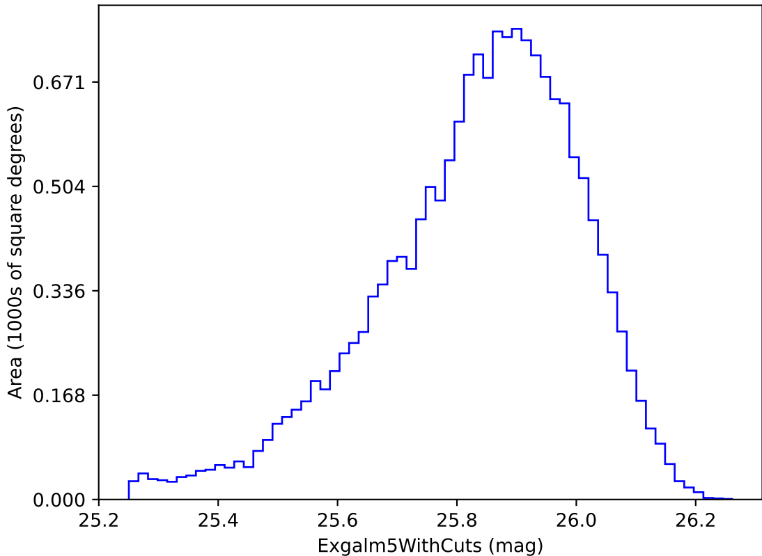
noroll_mjdp120_v3.4_10yrs i band non-DD year 3: ExgalM5WithCuts
