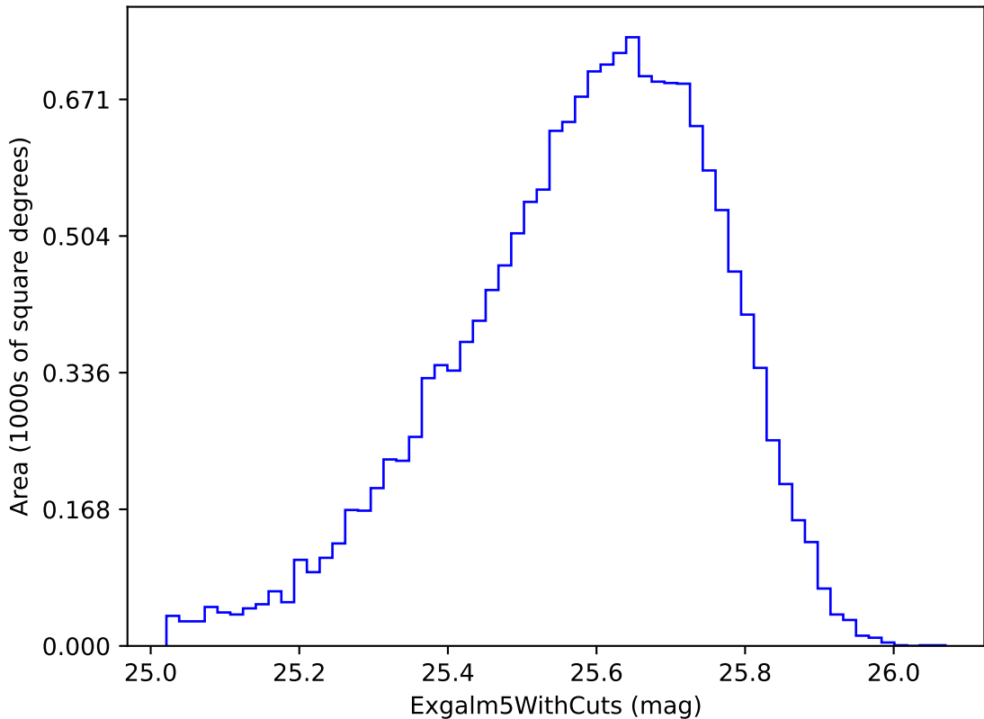
noroll_mjdp120_v3.4_10yrs i band non-DD year 2: ExgalM5WithCuts
