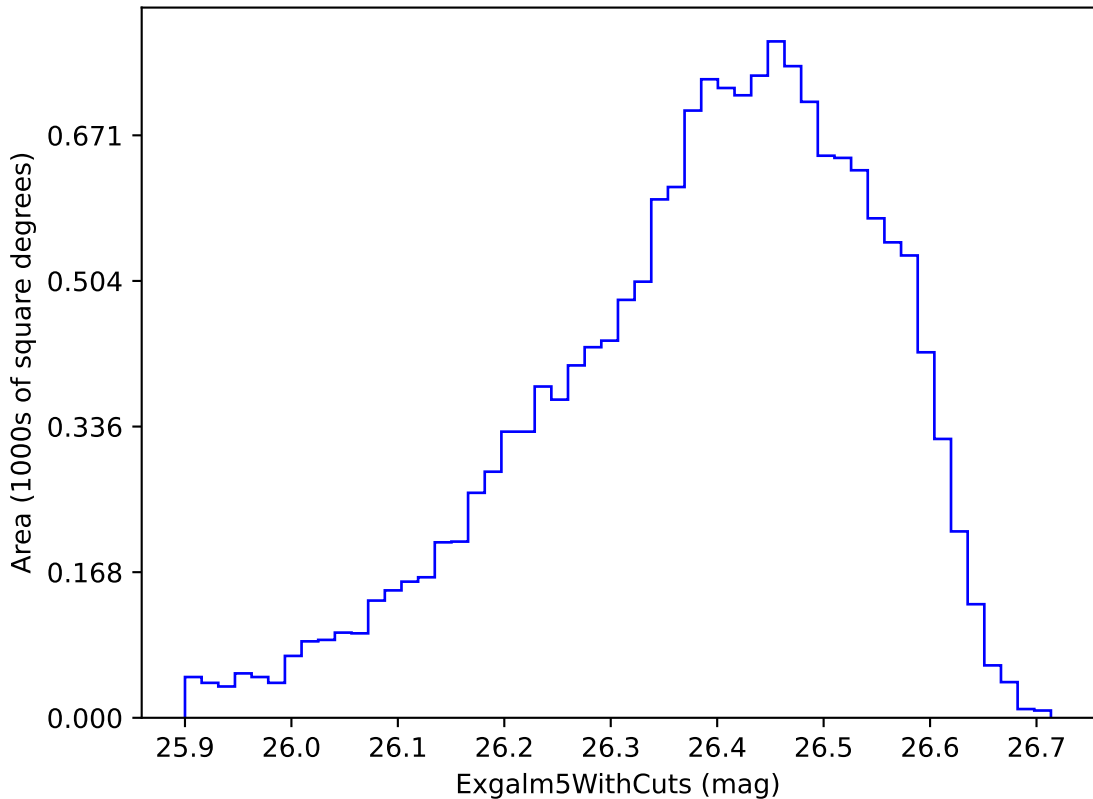
noroll_mjdp120_v3.4_10yrs i band non-DD year 10: Exgal5WithCuts
