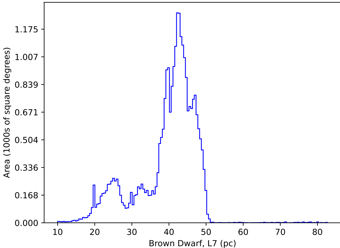
noroll_mjdp120_v3.4_10yrs : Brown Dwarf, L7
