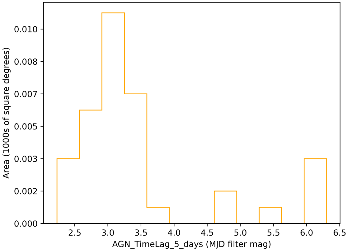
noroll_mjdp120_v3.4_10yrs r band: AGN_TimeLag_5_days
