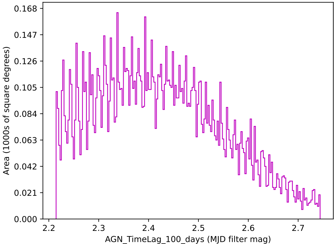
noroll_mjdp120_v3.4_10yrs z band: AGN_TimeLag_100_days
