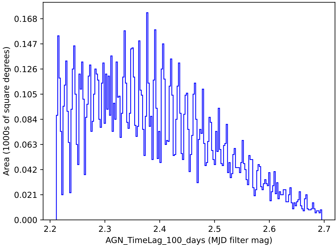
noroll_mjdp120_v3.4_10yrs y band: AGN_TimeLag_100_days
