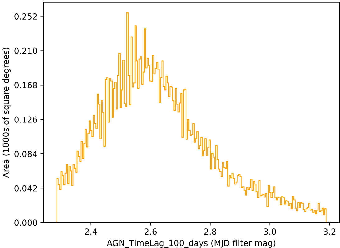
noroll_mjdp120_v3.4_10yrs r band: AGN_TimeLag_100_days
