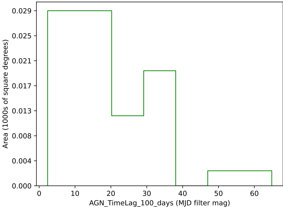
noroll_mjdp120_v3.4_10yrs g band: AGN_TimeLag_100_days
