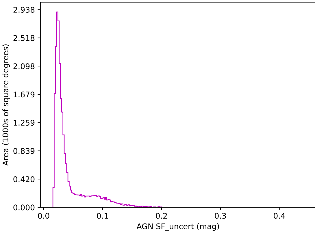
noroll_mjdp120_v3.4_10yrs z band: AGN SF_uncert
