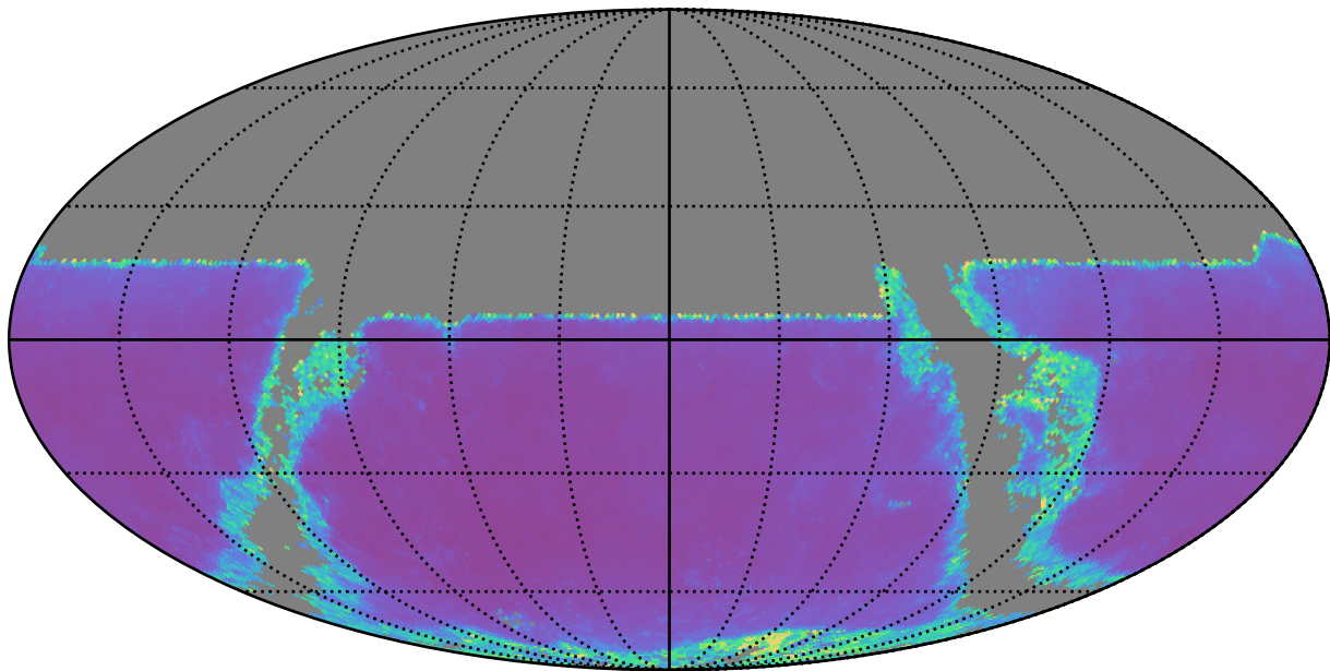
noroll_mjdp120_v3.4_10yrs y band: AGN SF_uncert
