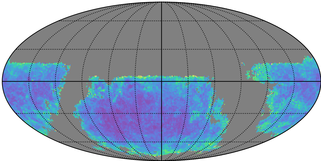
noroll_mjdp120_v3.4_10yrs u band: AGN SF_uncert
