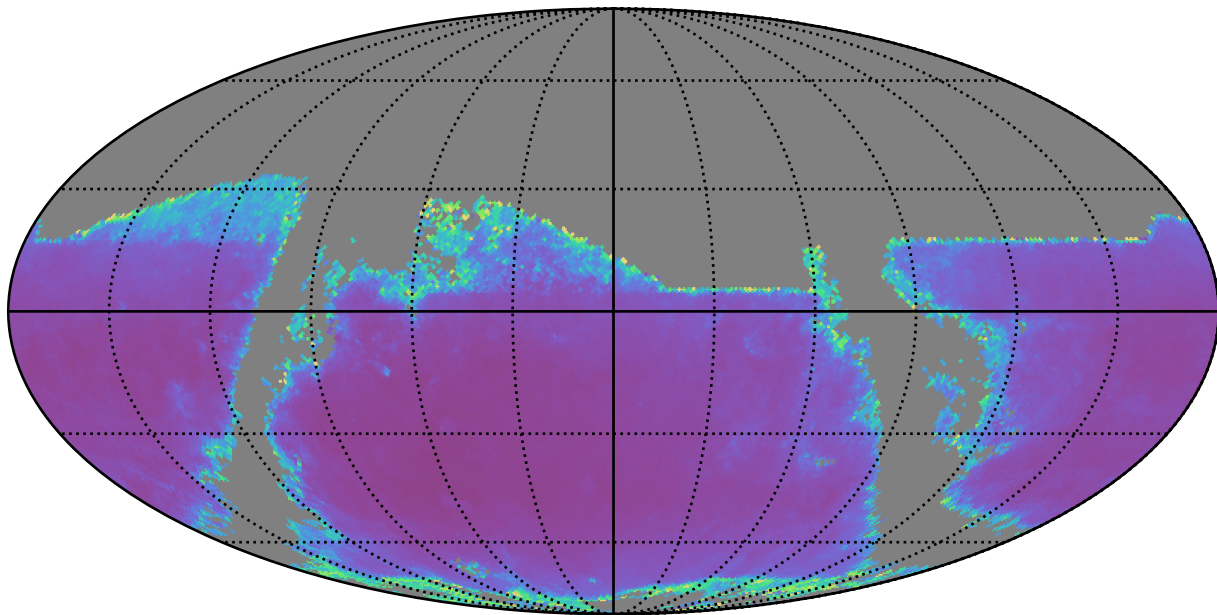
noroll_mjdp120_v3.4_10yrs r band: AGN SF_uncert
