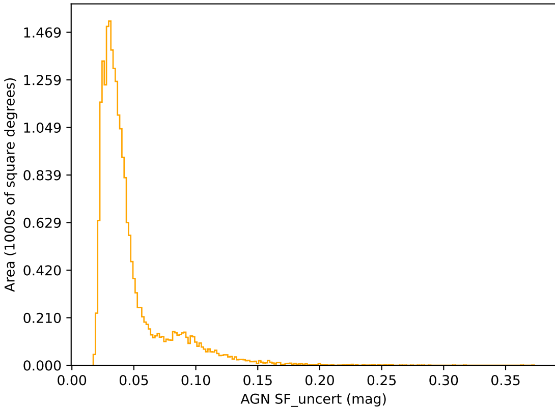
noroll_mjdp120_v3.4_10yrs r band: AGN SF_uncert
