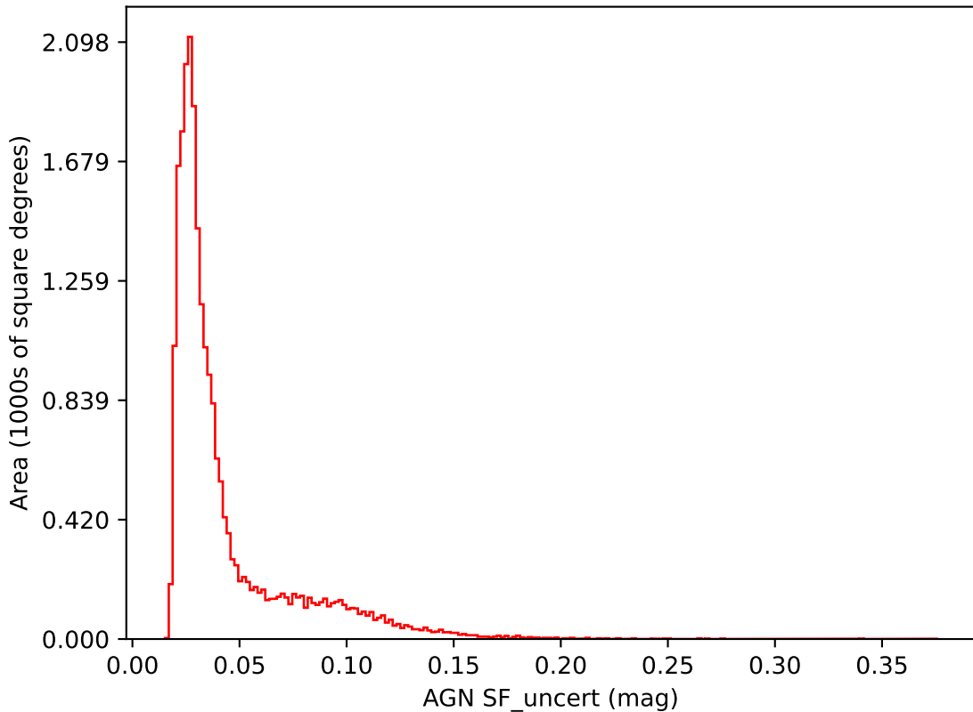
noroll_mjdp120_v3.4_10yrs i band: AGN SF_uncert
