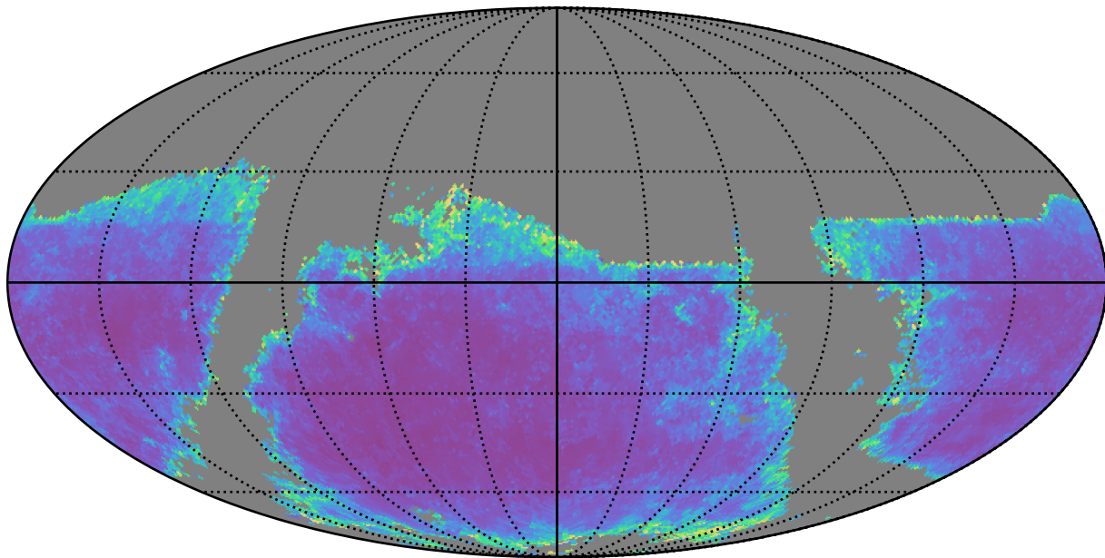
noroll_mjdp120_v3.4_10yrs g band: AGN SF_uncert
