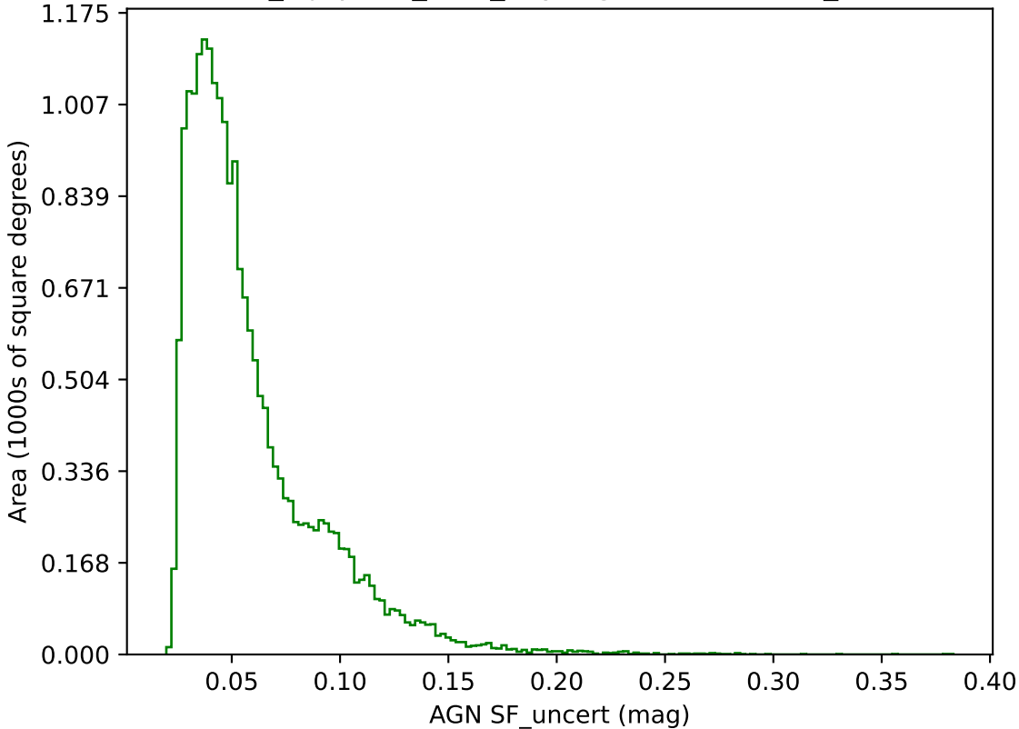
noroll_mjdp120_v3.4_10yrs g band: AGN SF_uncert
