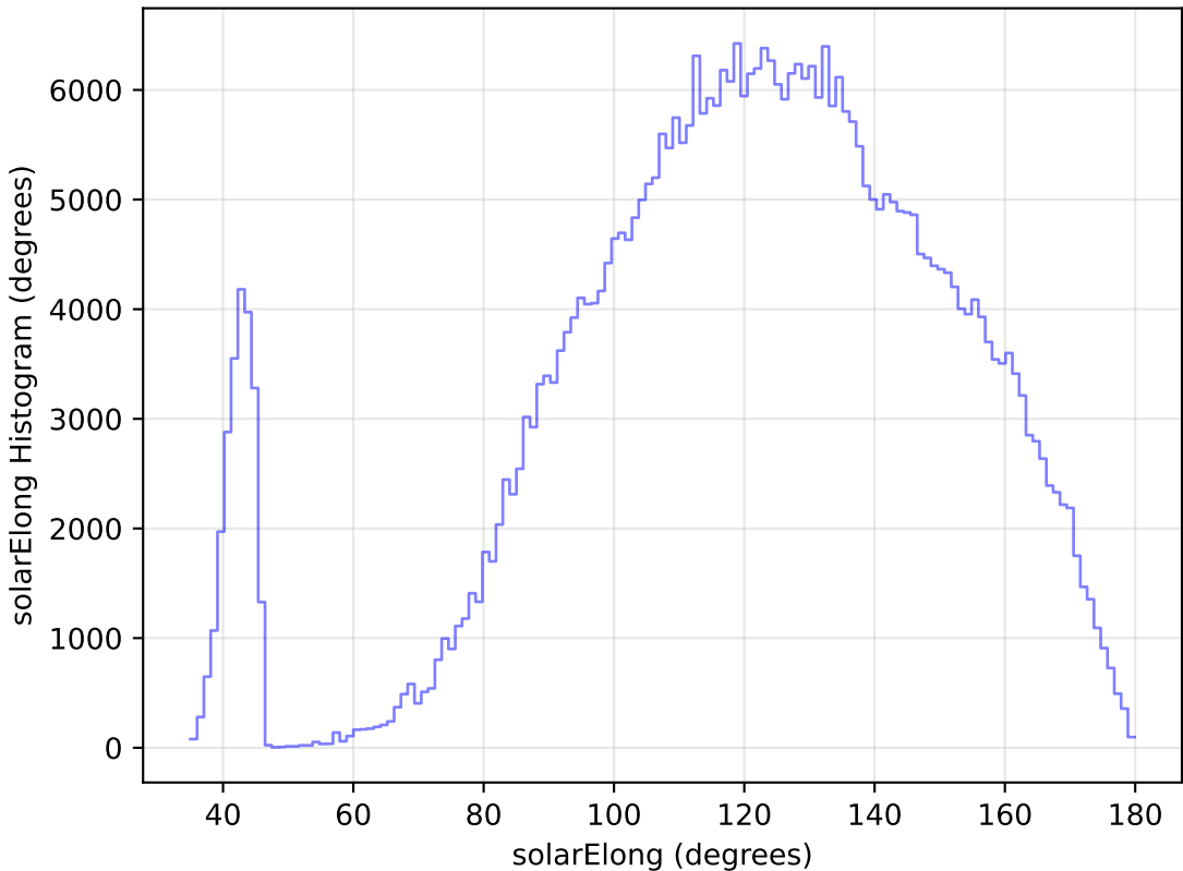
noroll_mjdp120_v3.4_10yrs WFD z band: solarElong Histogram
