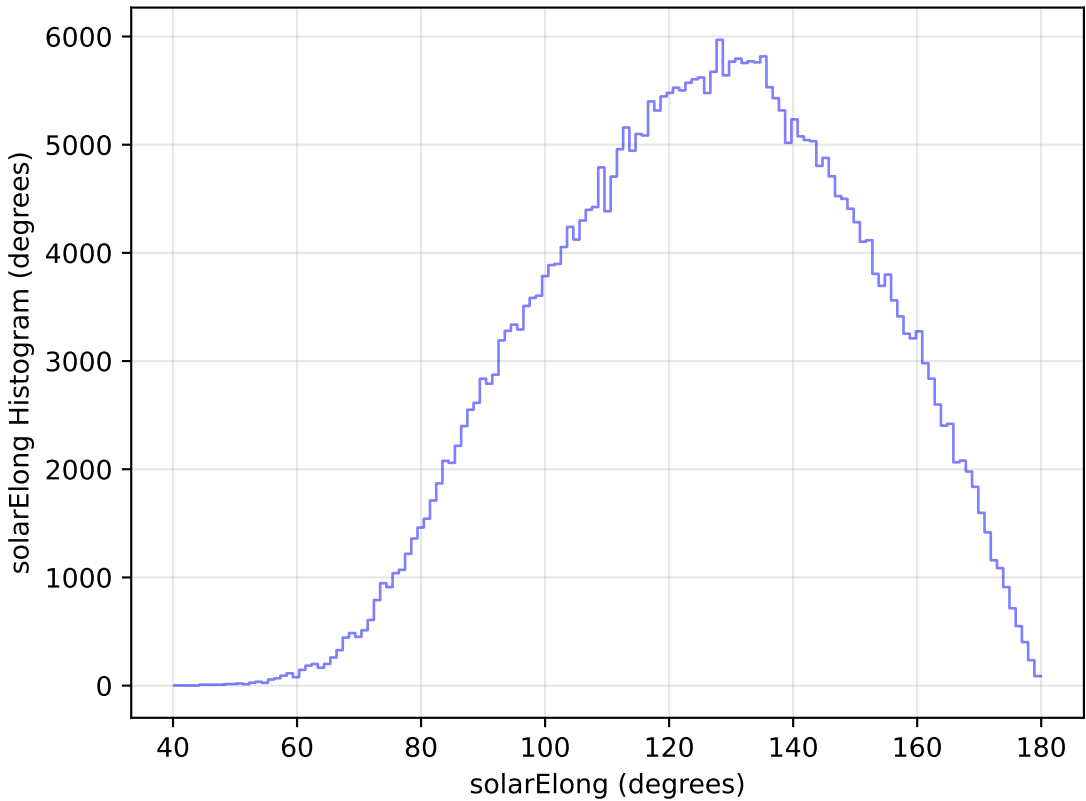
noroll_mjdp120_v3.4_10yrs WFD y band: solarElong Histogram
