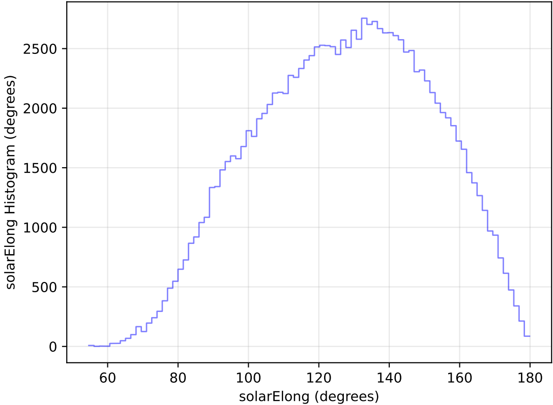
noroll_mjdp120_v3.4_10yrs WFD u band: solarElong Histogram
