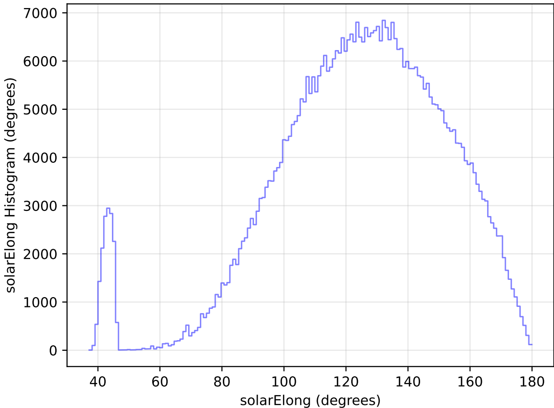
noroll_mjdp120_v3.4_10yrs WFD r band: solarElong Histogram
