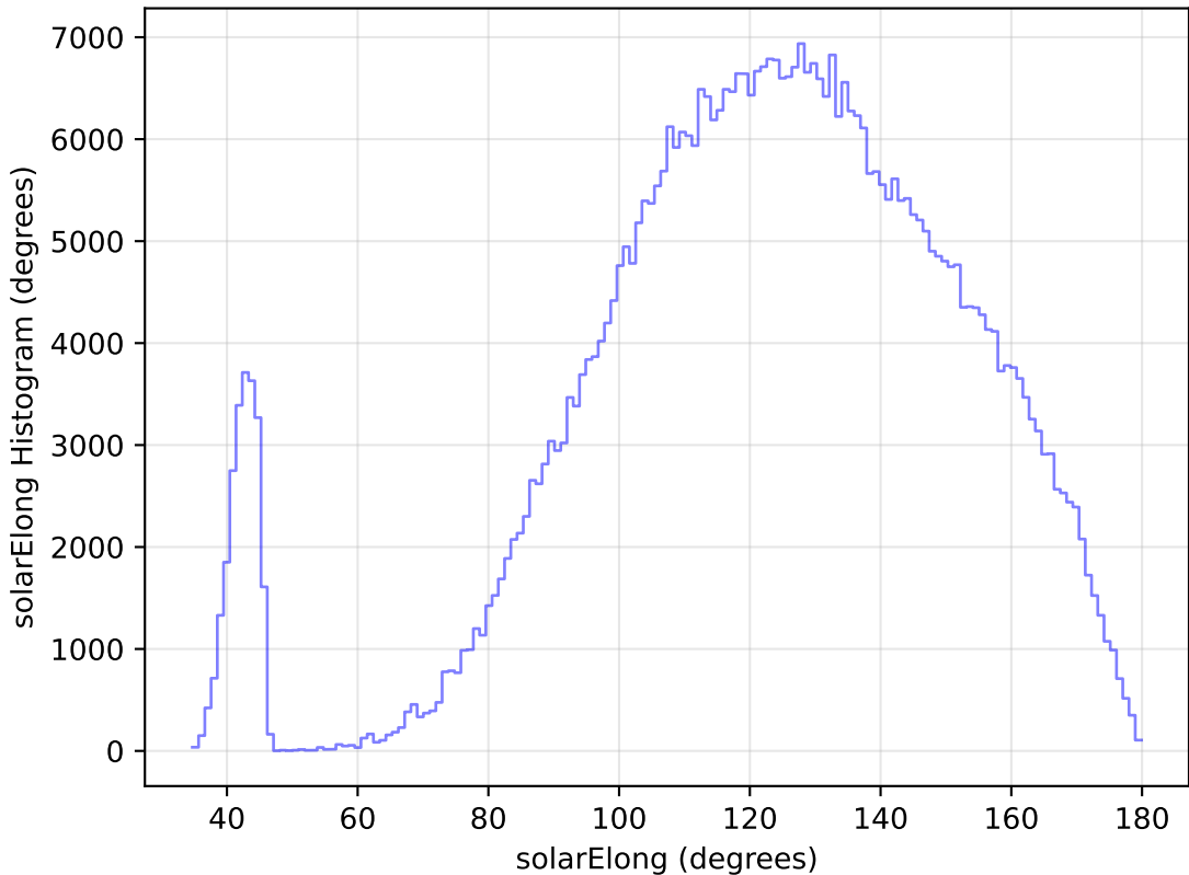
noroll_mjdp120_v3.4_10yrs WFD i band: solarElong Histogram
