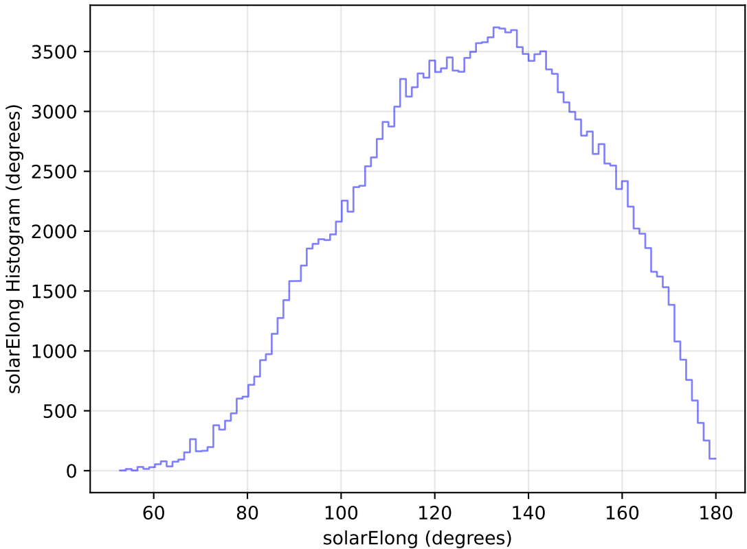
noroll_mjdp120_v3.4_10yrs WFD g band: solarElong Histogram
