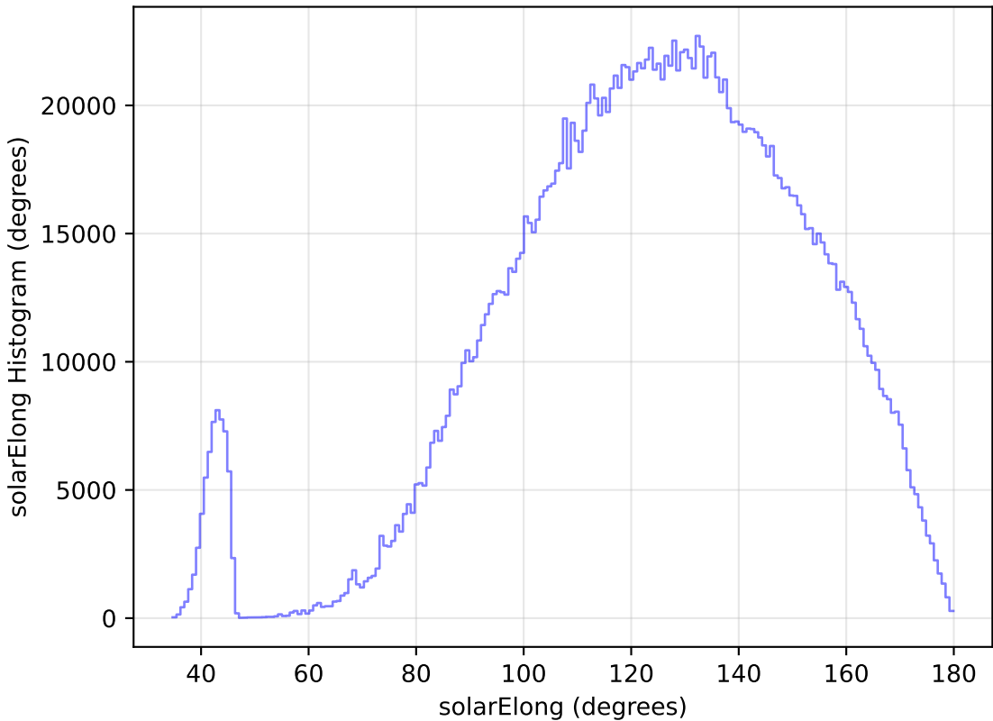
noroll_mjdp120_v3.4_10yrs WFD all bands: solarElong Histogram
