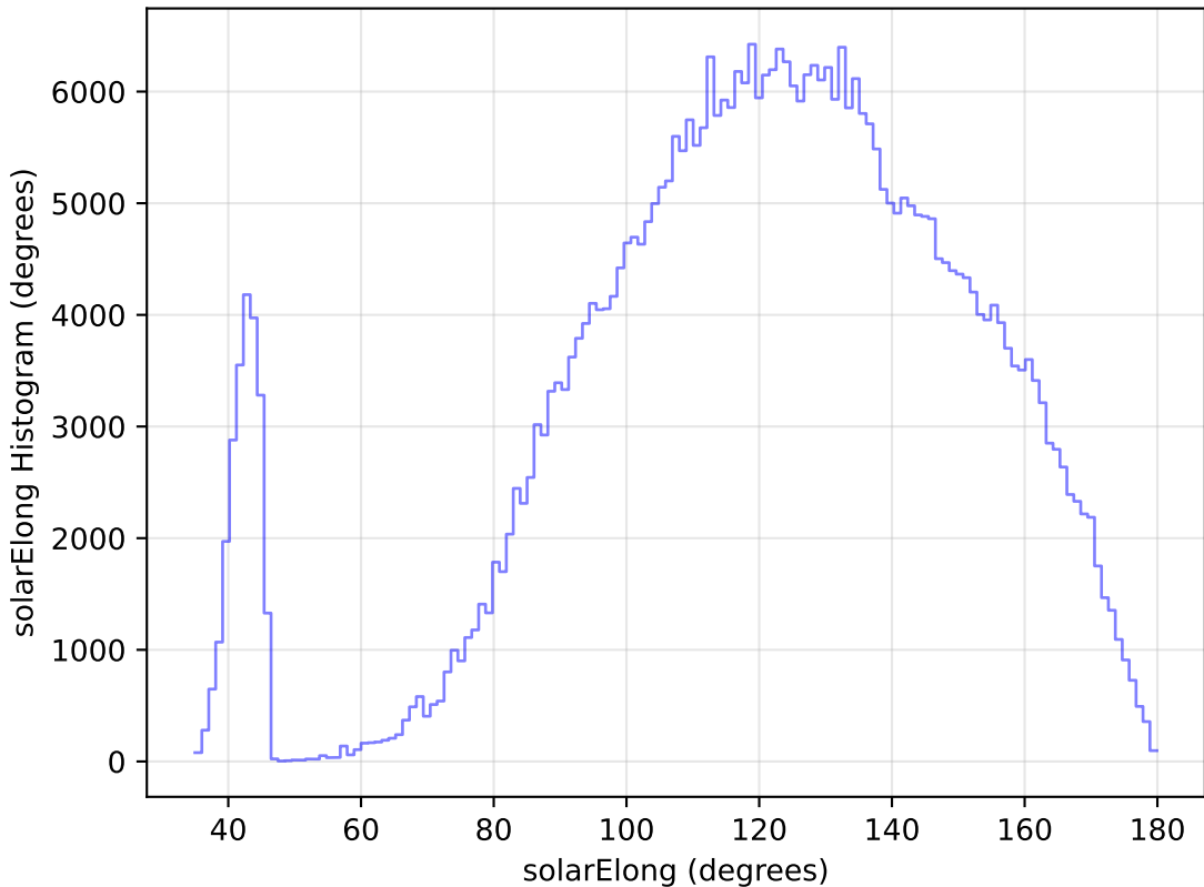
noroll_mjdp120_v3.4_10yrs All sky z band: solarElong Histogram
